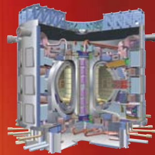
ITER cutaway
